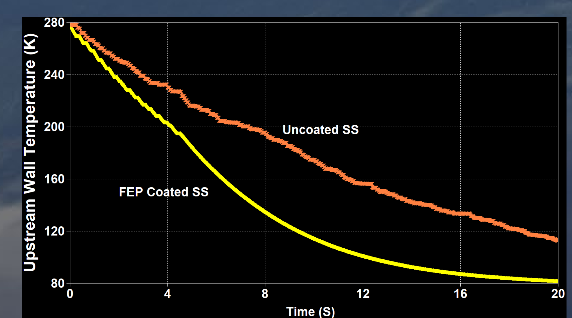
Comparison of a microfilm coated line and an uncoated line during continuous flow line chilldown.
