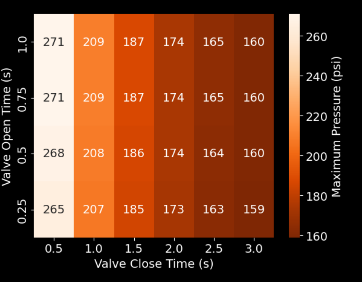
(2) Heat map of pressure spikes versus valve open and close times
