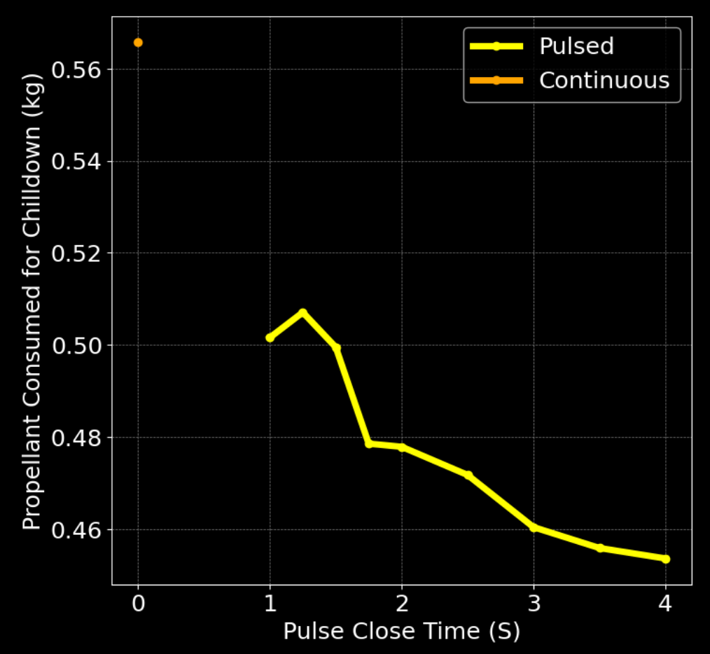
(1) Propellant consumed vs time the valve is closed for.
