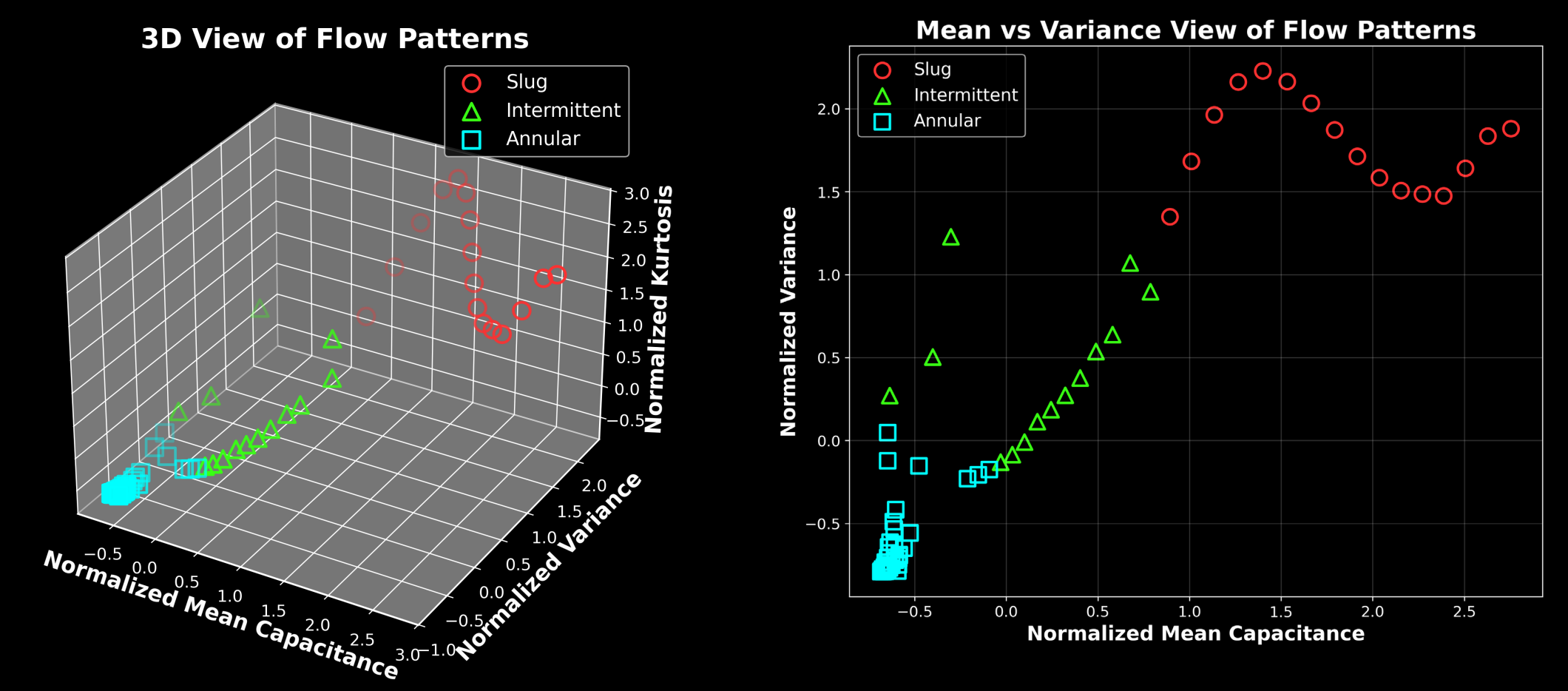
3-D visualization of flow regime map
