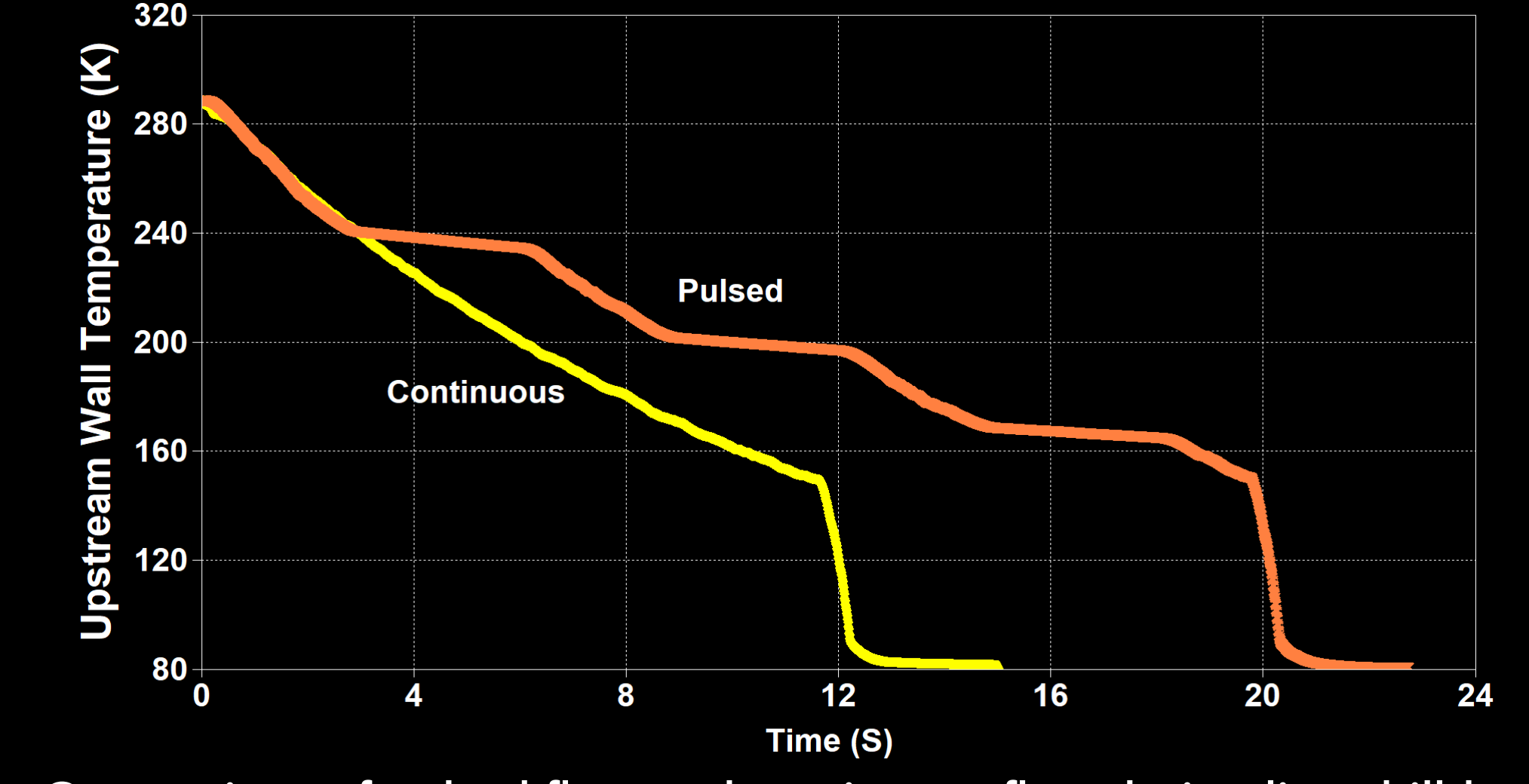
Comparison of pulsed flow and continuous flow during line chilldown
