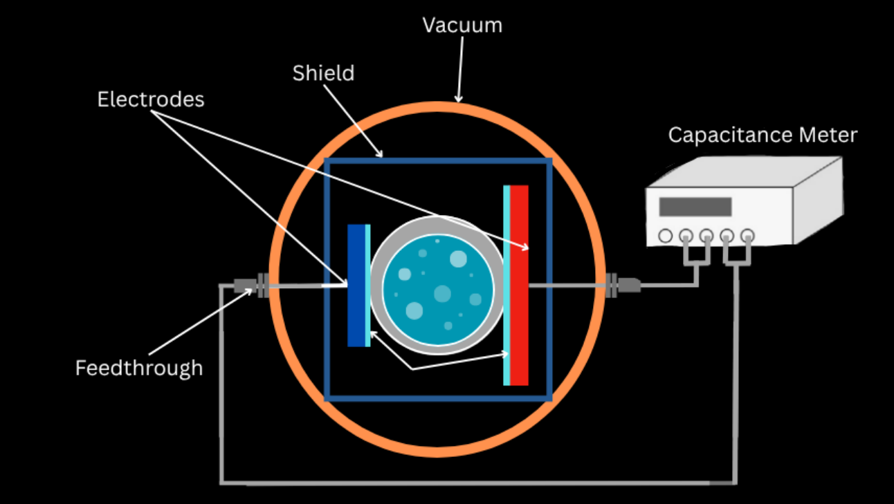
Sensor Depiction on Transfer Pipe
